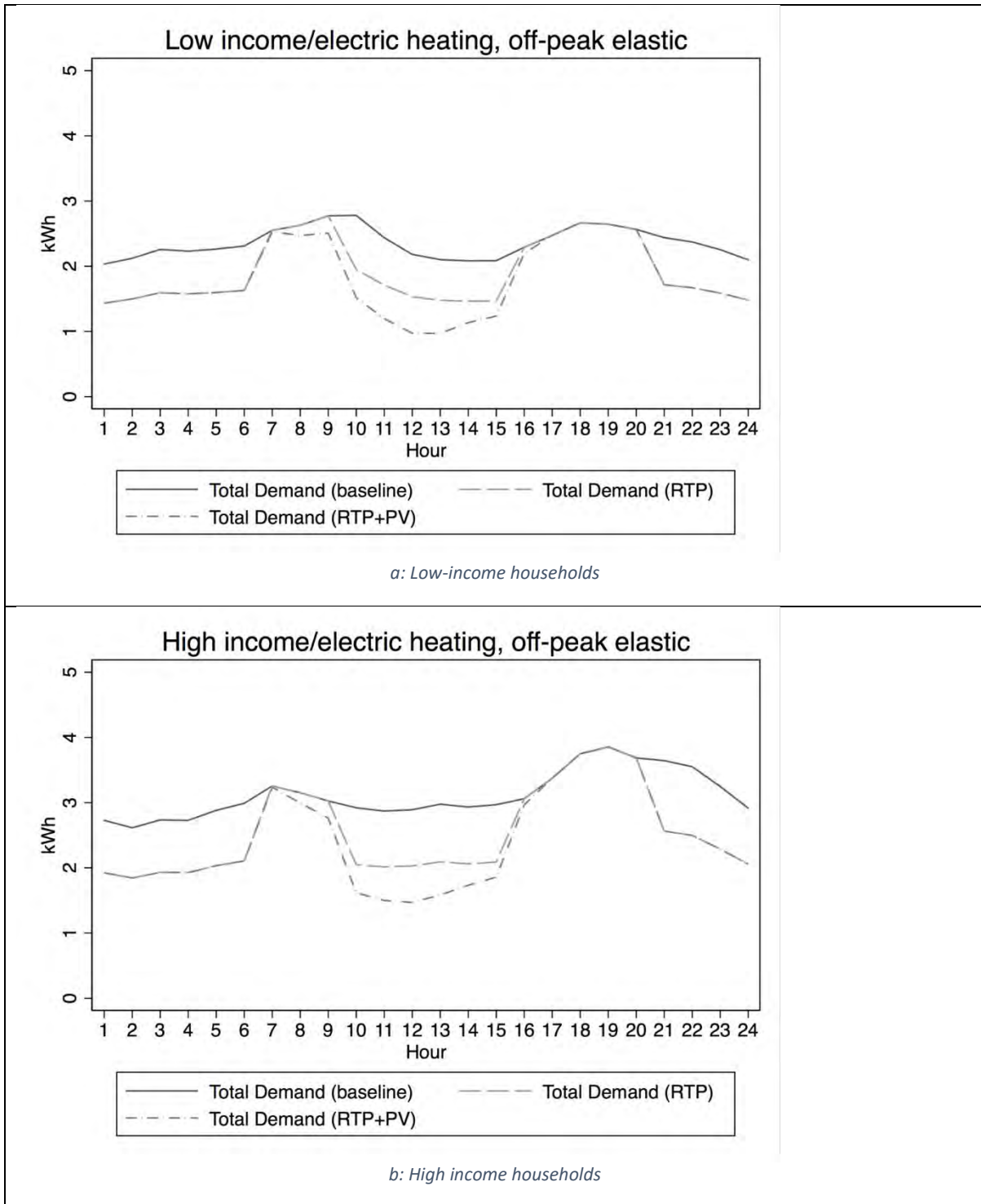
Figure 9: RTP-b for electrically heated households
