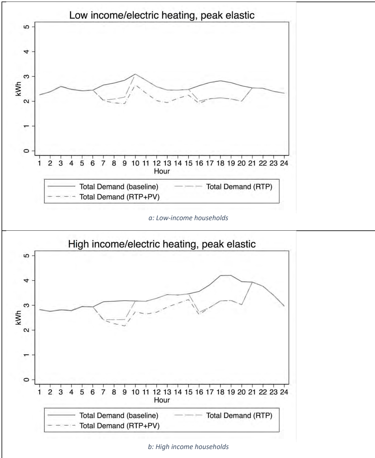
Figure 10: RTP-a for electrically heated households
