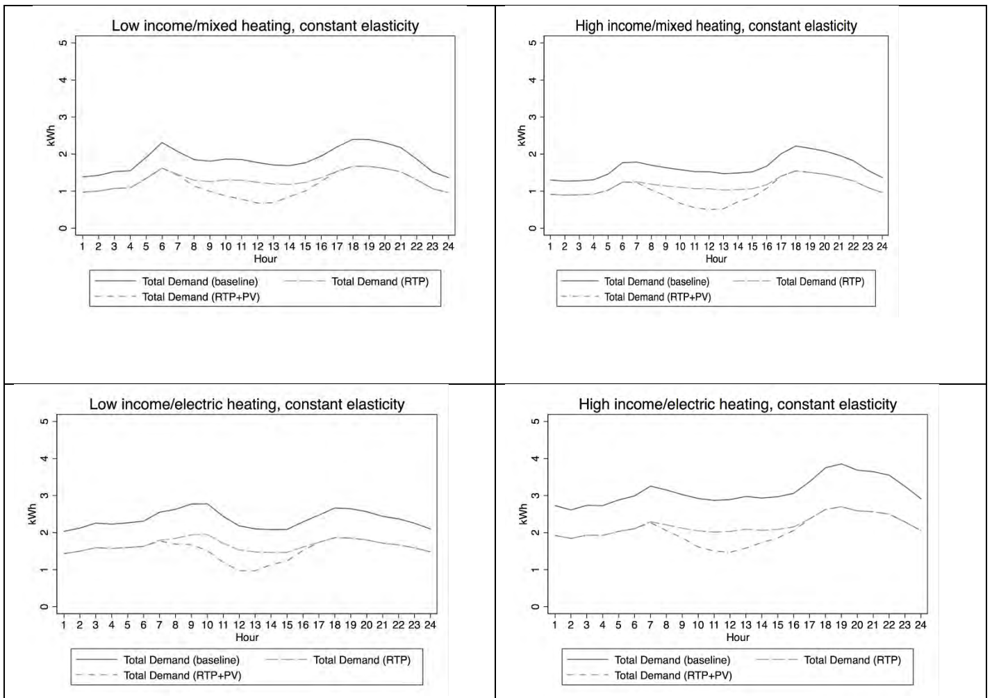
Figure 7: Constant Elasticity Loads.
